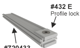
#720433 Reinforcing profile
