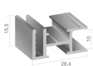
720421 Miniframe 15.5 mm
